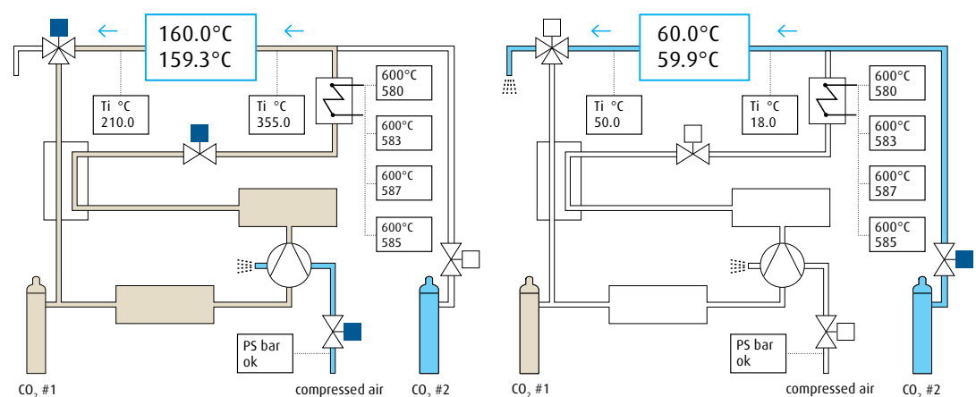
Heating process
